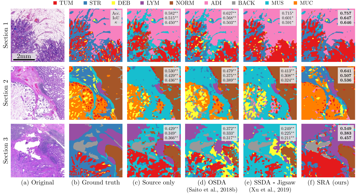
Figure 3: Examples of domain adaptations from K19 to our in-house dataset. (a-b) show the original sections from the WSIs and their ground truth, respectively. We compare the performance of our Self-Rule to Adapt (SRA) algorithm (f) to the lower bound and the previous top methods (c-e). We report the pixel-wise accuracy, the weighted intersection over union, and the pixel-wise Cohen’s kappa ( \kappa ) score.
