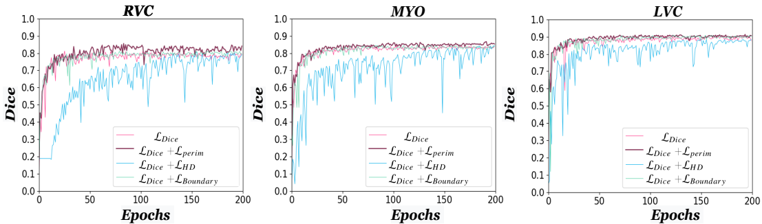
Figure 4: Curve evolution of Dice index on the three cardiac structures of the ACDC dataset in the multi-label segmentation. RVC/LVC: right/left ventricular cavity, MYO: myocardium
