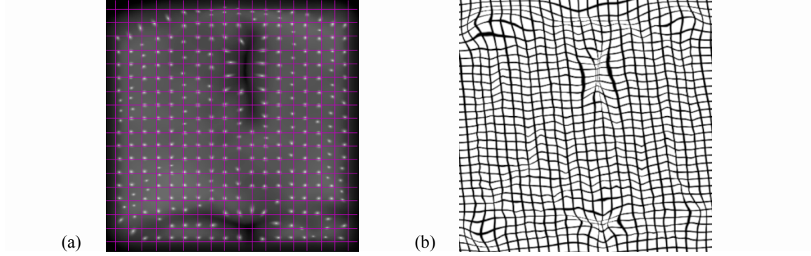
Figure A.1: Failed registration using ANTs. (a) morphed image, (b) deformation field.
