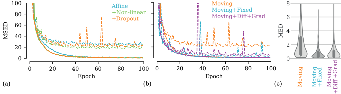
Figure 3: Feature-based registration on a synthetic dataset. (a) MSE loss of training (solid line) and validation (dashed line) set across training epochs for different transformation settings (T1-T3). (b) MSE loss of training (solid line) and validation (dashed line) set across training epochs for different inputs (T3, I2, I3). Same y-axis as in panel (a). (c) Distribution of mean Euclidean distances (MEDs) for different inputs on the validation set (T3, I2, I3).
