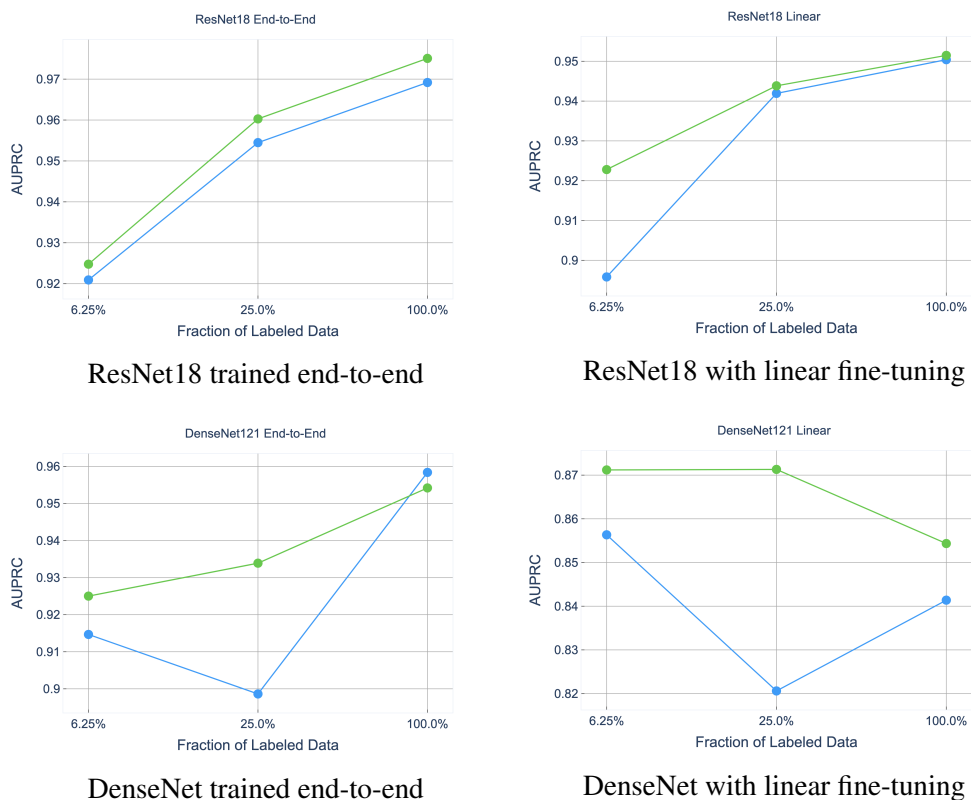
Figure 4: Comparison of AUPRC performances for ResNet18-based and DenseNet121-based models on the tuberculosis task from the Shenzhen dataset.
